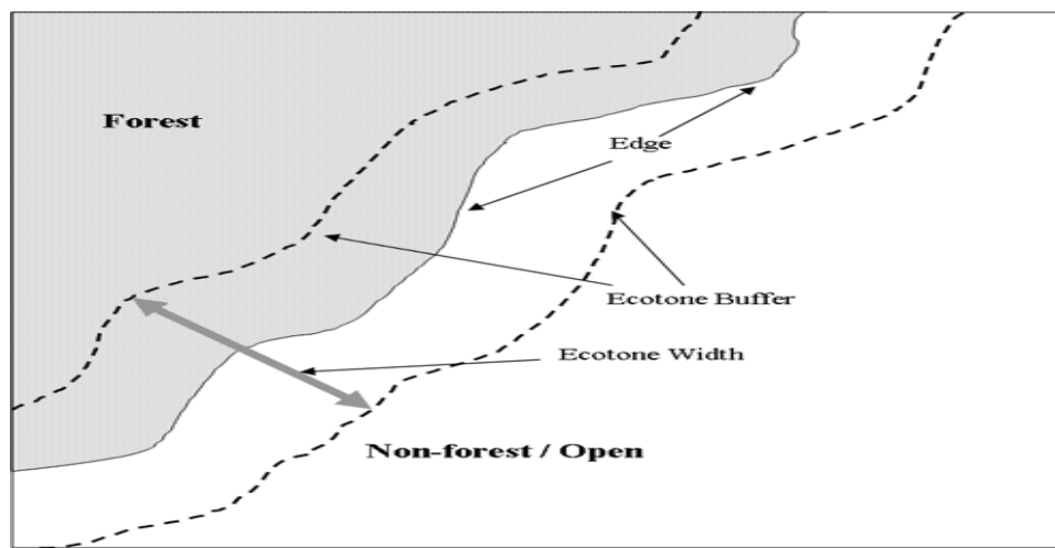
Figure 10: A transition zone or ecotone
