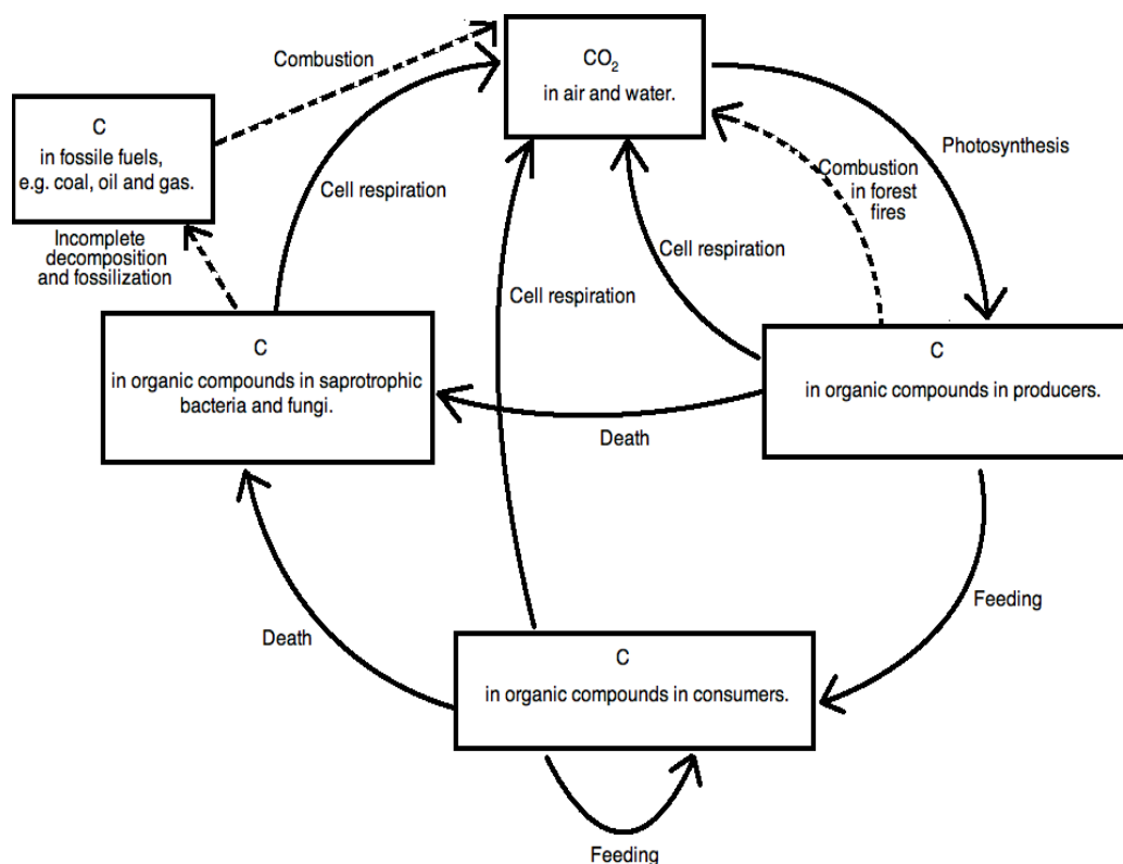
Figure 16: Carbon cycle
