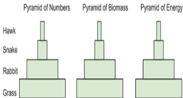
Figure14: Ecological pyramids
