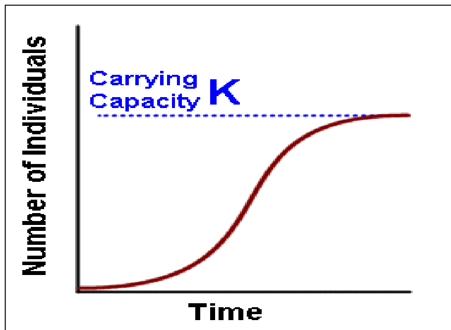
Figure 9: S-shaped growth curve
