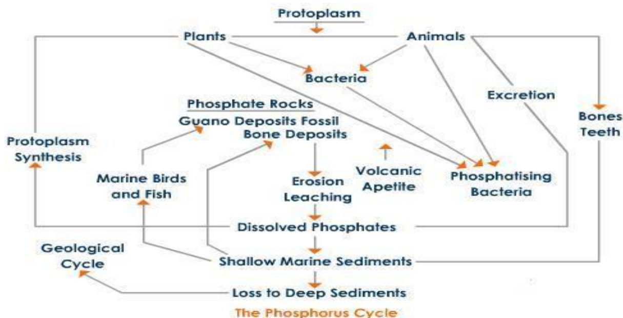
Figure 18: Phosphorus cycle
