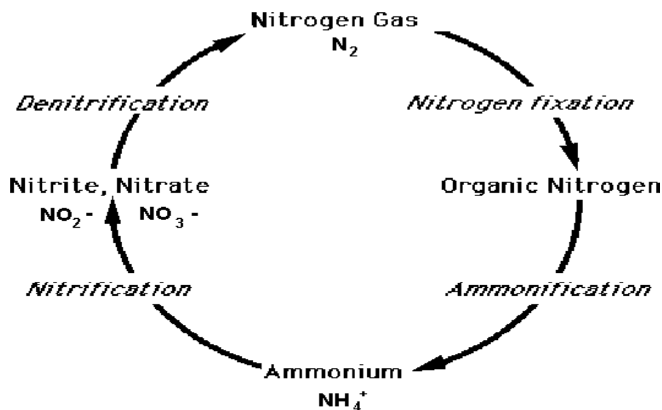
Figure 17: Nitrogen cycle
