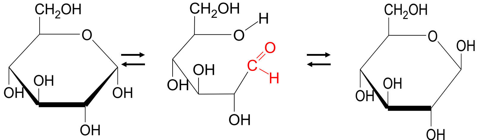
\alpha -D-glucose (36%)
