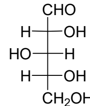
D-xylose
