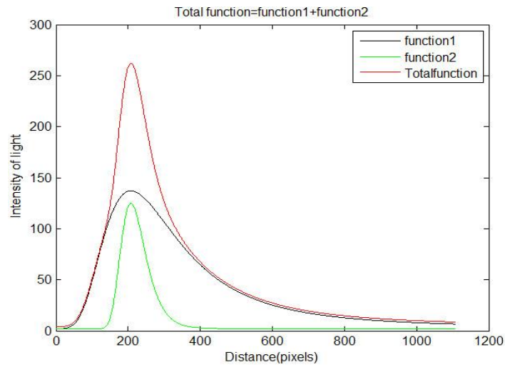
Fig. 5: Red curve which identical with original curve of comet is consist from two function ,black curve and green curve.
