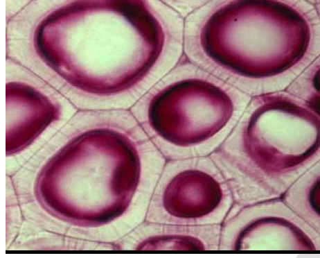
Diospyros endosperm
