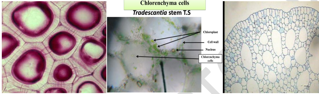
Storage parenchyma
