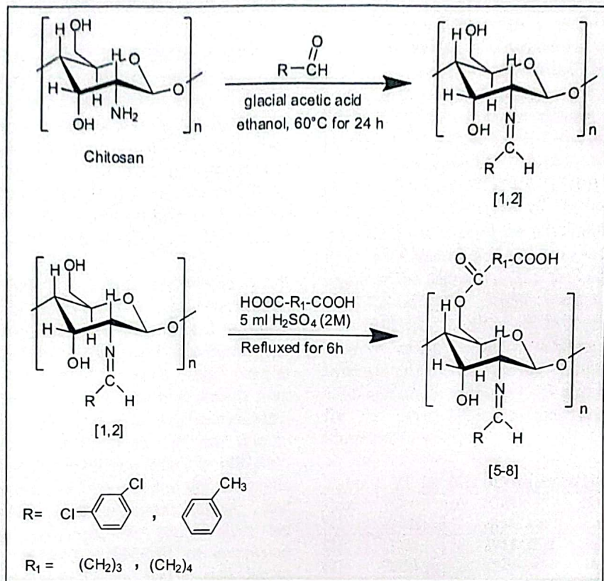
Scheme 1. Synthesis of polymers [1-2], [5-8]
