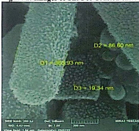
(A): Image of polymer(5) blend with PVA
