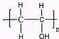
Figure 1. Structure of Polyvinyl alcohol(PVA)
