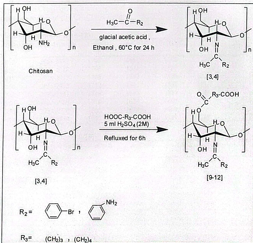
Scheme 2. Synthesis of polymers [3-4], [9-12]
