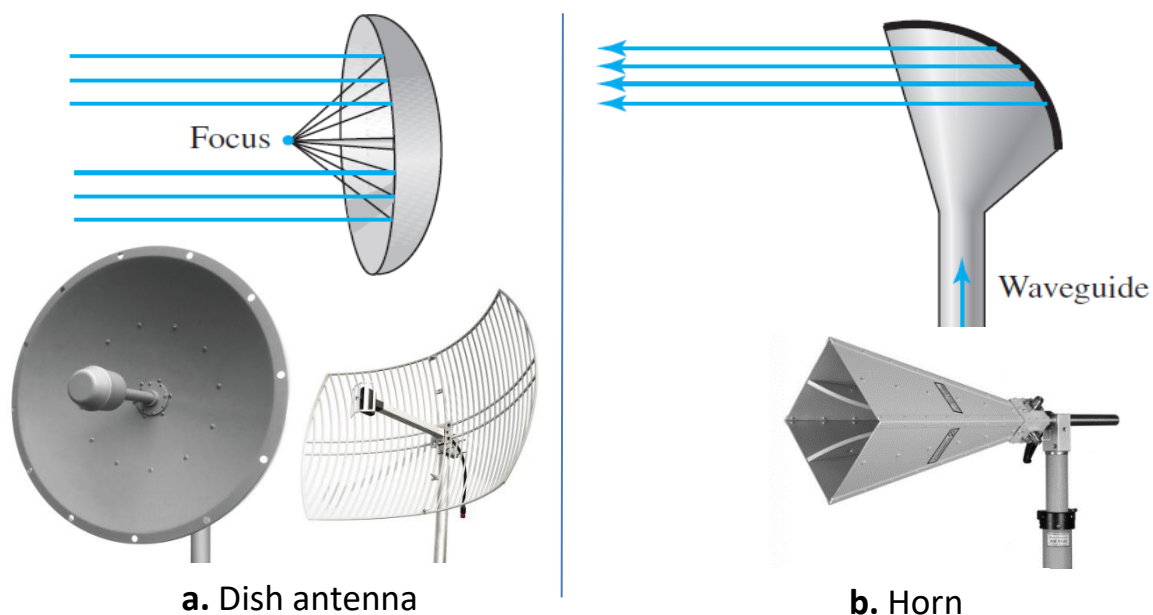
Figure 6.11 Unidirectional antennas
