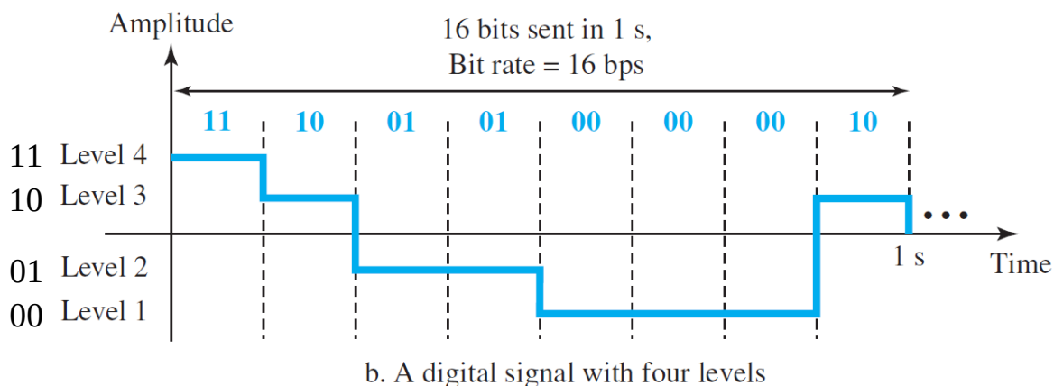
Figure 5.1 Two digital signals: one with two signal levels and the other with four signal levels
