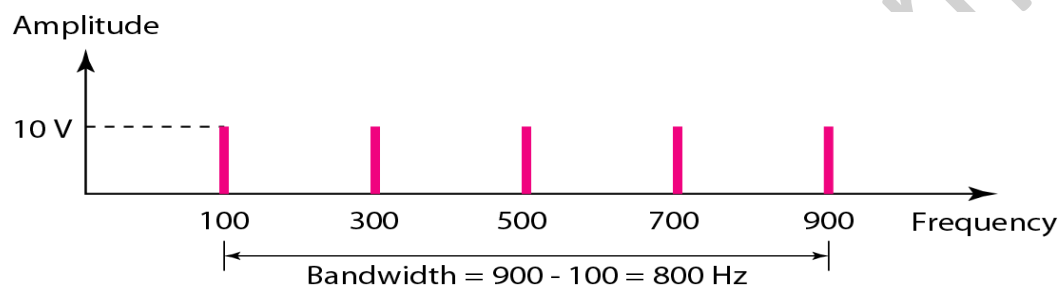
Figure 4.9 The bandwidth for Example 4
