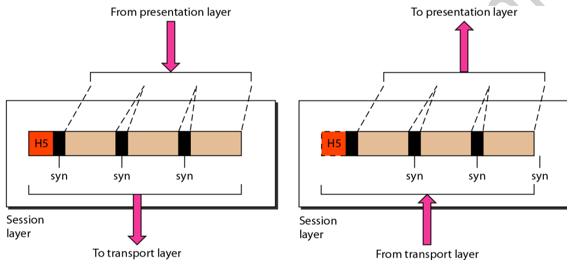
Figure 2.8 Session layer
