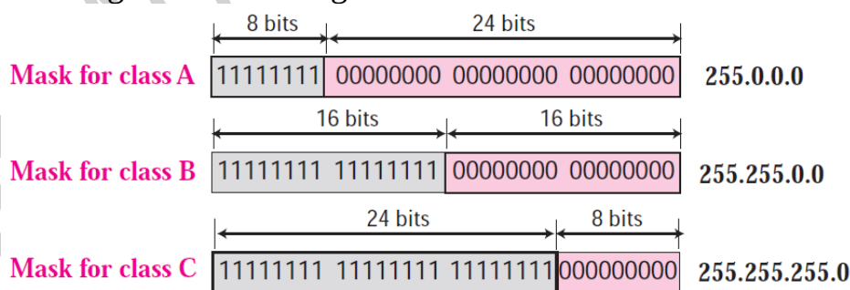
Figure 7.10 Network mask
