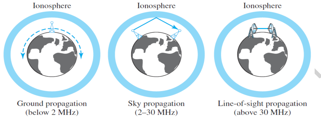
Figure 6.9 Propagation methods
