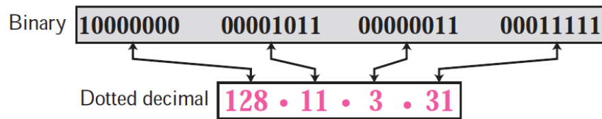
Figure 7.1 Dotted-decimal notation
