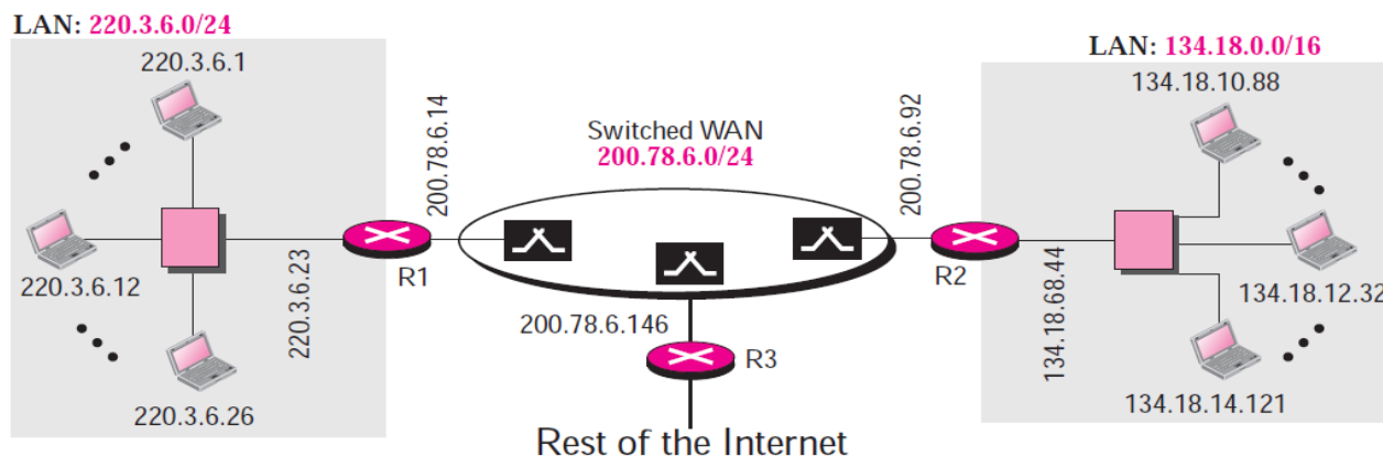
Figure 7.9 Sample internet
