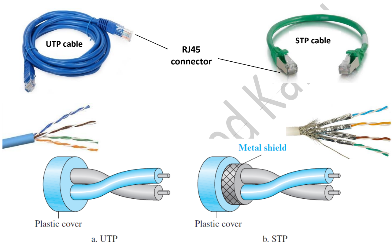
Figure 6.4 UTP and STP cables
