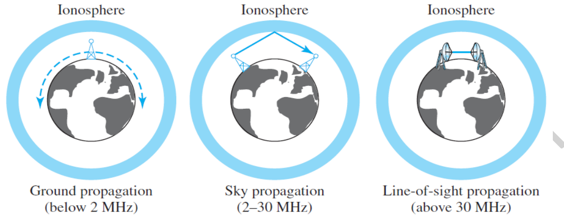
Figure 6.9 Propagation methods
