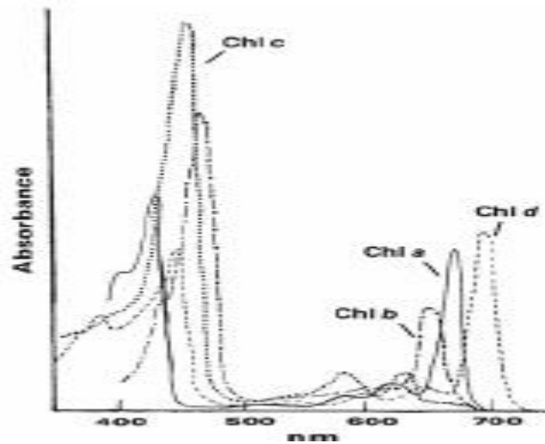
Figure 1-19: The Absorption spectra of chlorophyll a, b, c, and d
