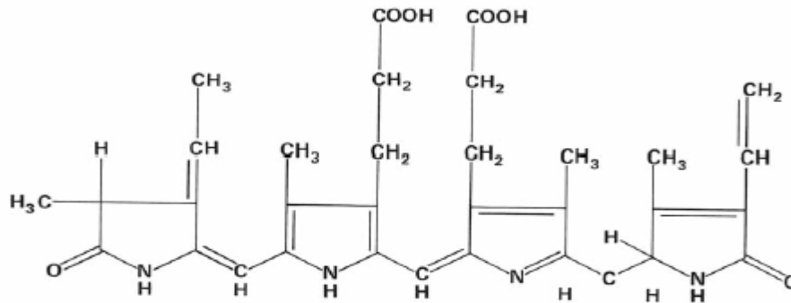
Fig. 1.22 The structure of phycoerythrobilin.
