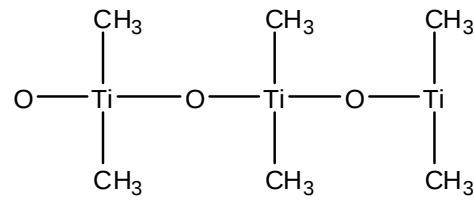
Polydimethyltitanoxane
