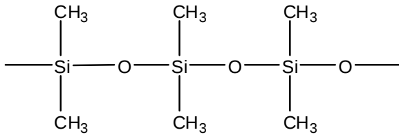
Polydimethylsiloxane
