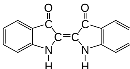
Indigo (Cis-form)
