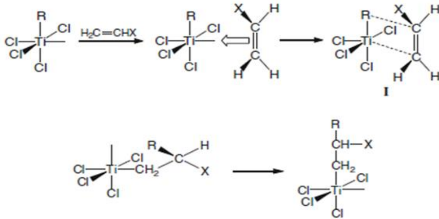
Monometallic mechanism of Ziegler-Natta polymerization of substituted alkene
