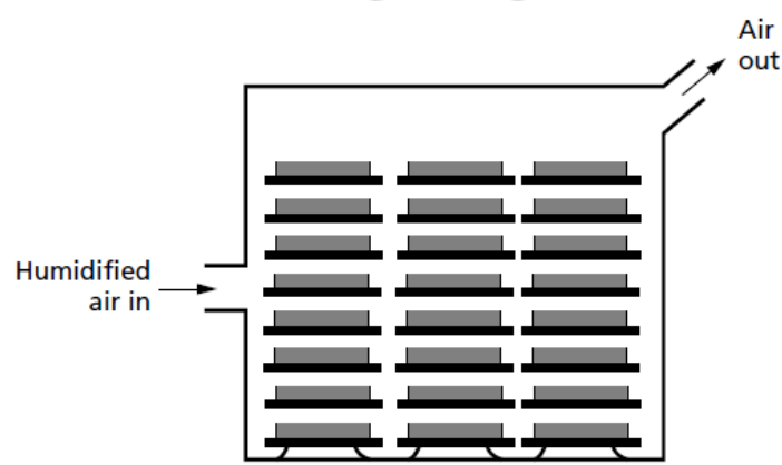
Figure: Tray fermentor
