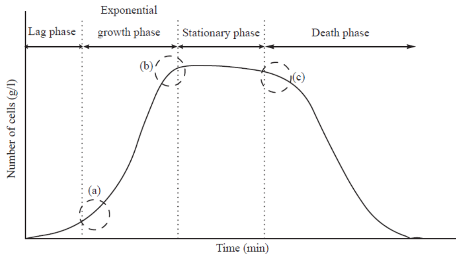
Figure: Growth curve of a batch culture. (a) Acceleration phase, (b) Retardation phase and (c) Declining phase.
