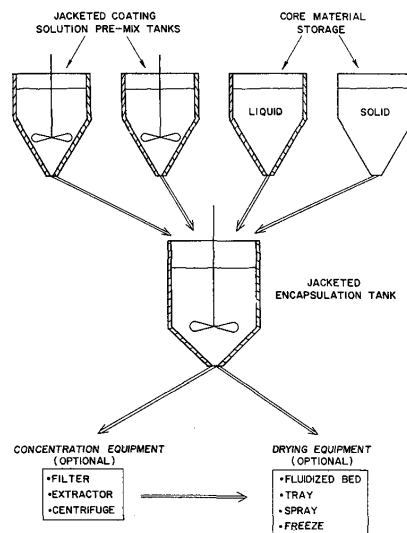
FIG. 13-44. Flow diagram of a typical phase-separation/coacervation process. (From Bakan. 26 )
