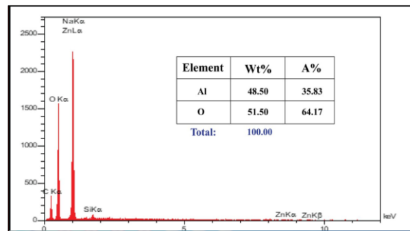
Figure 8. EDX of \gamma - \text{Al}_2\text{O}_3 NPs powder from aqueous extract of clove.
