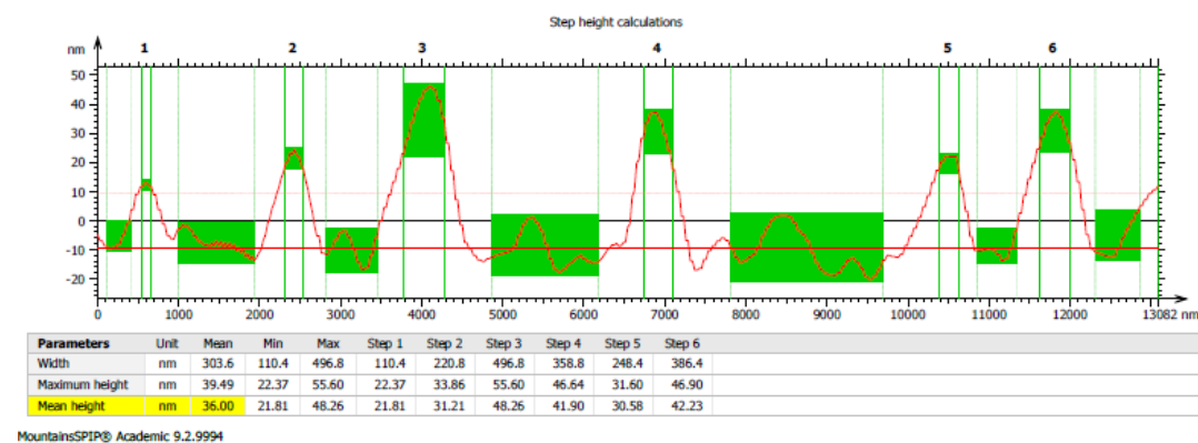
Figure 11. (a) AFM curve of particle analysis length of \gamma - \text{Al}_2\text{O}_3 NPs powder, (b) AFM height and width calculations parameters of \gamma - \text{Al}_2\text{O}_3 NPs powder.
