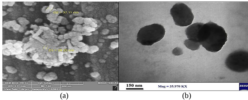
Figure 7. (a) Images of SEM and (b) TEM of \gamma - \text{Al}_2\text{O}_3 NPs powder.
