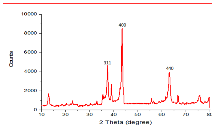
Figure 6. XRD of \gamma\text{-Al}_2\text{O}_3 NPs powder from aqueous extract of clove.
