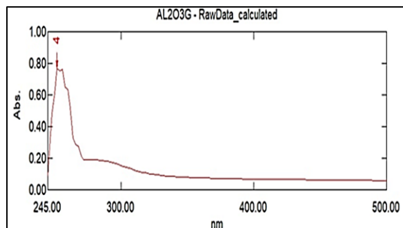
Figure 5. U.V- vis spectrum of \gamma\text{-Al}_2\text{O}_3 NPs from aqueous extract of clove.
