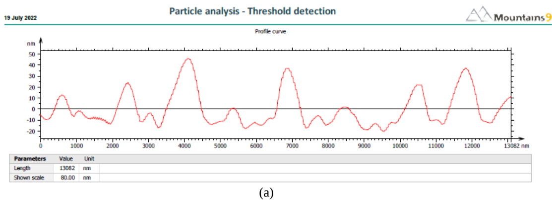
Figure 10. AFM histogram and statistical particle analysis of \gamma - \text{Al}_2\text{O}_3 NPs powder.
