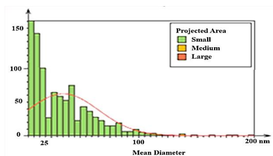
Figure 9: AFM histogram and statistical particle analysis of CaONPs powder.
