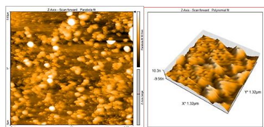
Figure 10: 3D AFM surface structure images of CaONPs.
