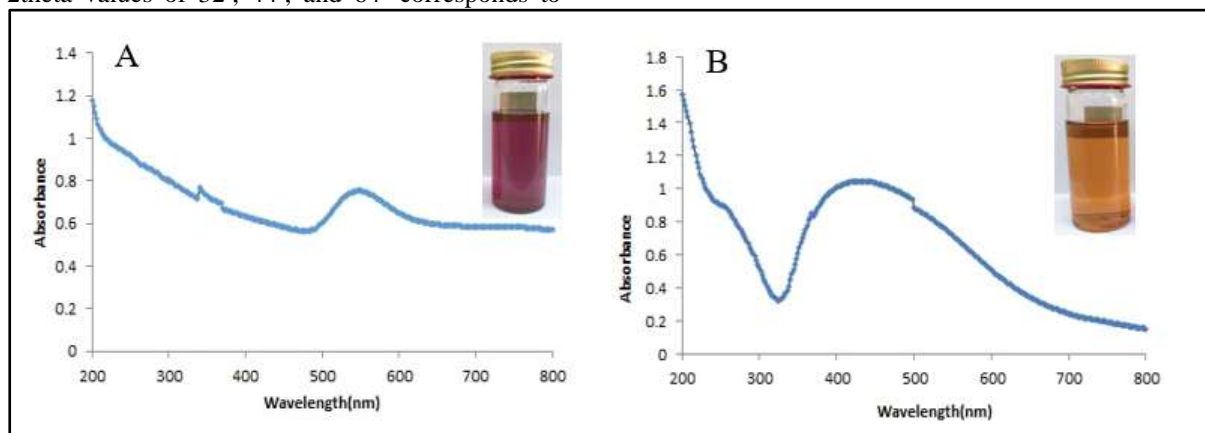
Figure. 2. UV-Vis spectrum of A- AuNPs and B- AgNPs (31) .
