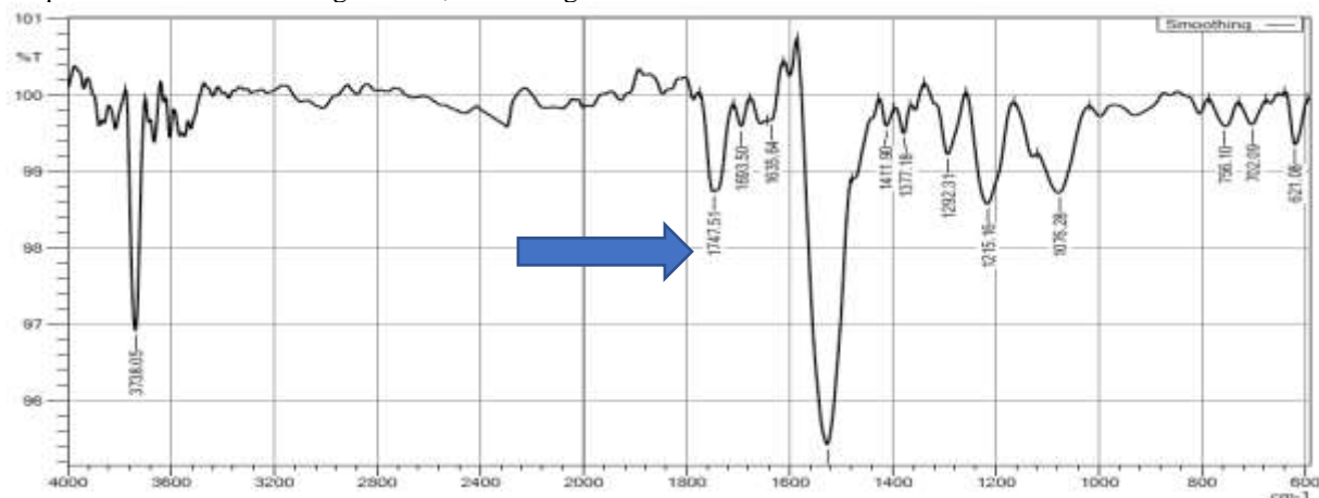
Figure. 4. FTIR Spectrum of chitosan Schiff base
