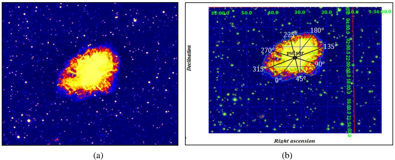
Fig. 1: a: Image of Crab nebula taken from SAO-DSS [14] b: image (a) after locate the pulsar position on it and divided into eight regions with constant angle.
