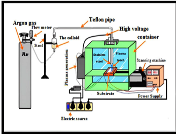
Figure 1. The Schematic Diagram of the Plasma Jet System
