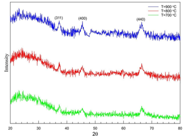
Figure 7. XRD Patterns for Al 2 O 3 Films After Annealing at Different Temperatures
