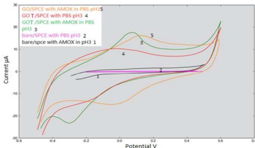
Figure: (13) Cyclic voltammogram of 0.5mM AMOX in 0.1M PBS (pH 3.0) at scan rate 0.1\text{v.s}^{-1} at bare and GO-T-Nafion/SPCE.
