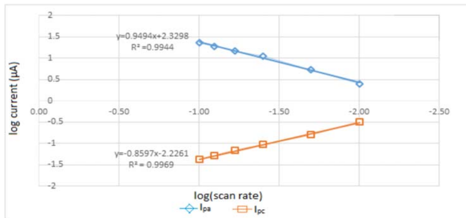
Figure: (17) Log current vs. log v for GOT modified SPCE in presence AMOX.
