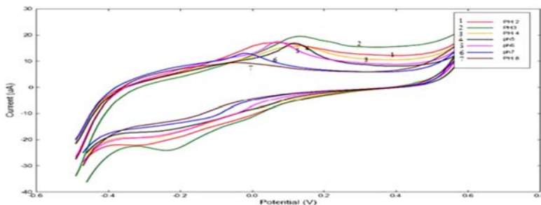
Figure: (10) Cyclic voltammogram obtained at GOT-Nafion/ SPCE with 0.5mM AMOX in PBS with different pH values at scan rate 0.1\text{v.s}^{-1} .
