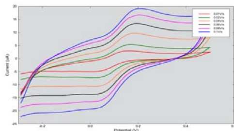
Figure: (9) Cyclic voltammogram for GOT-SPCE in potassium ferricyanide
