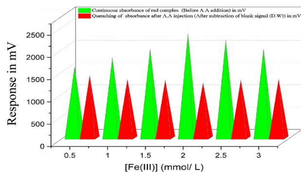
Fig. 3 Effect of ferric ion concentration using \text{Fe}^{3+} (variable concentration)– \text{SCN}^- (2 \text{mmol L}^{-1} )– \text{H}_2\text{O} system and [\text{A.A}] = 38 \text{ mmol L}^{-1} on absorbance of complex formation, quenching sensitivity by ascorbic acid and the optimal concentration of ferric ion = 2.0 \text{mmol L}^{-1} .
