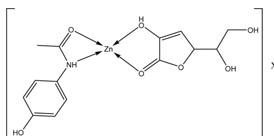
Fig. 13. The structure of PAPA-Asc complex. M = Cu..... X = Cl 2 , M = Zn .....X = SO 4
