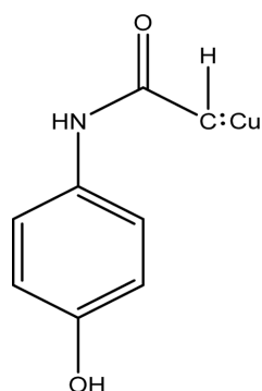
Fig. 11. The (Cu) was able to coordinate with (PAPA) via CH 3 -group.
