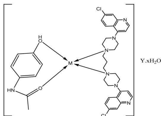
Fig. 14. M-(PQ)( PAPA): Where M(II) = Zn, Cu, Ni, Co and Fe. Y = Cl 2 , (CH 3 COO) 2 , or SO 4
