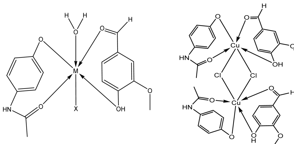
Fig. 6. The structures for Metal(II) complexes. M : Mn^{2+}, Co^{2+}, Ni^{2+}, and Zn^{2+} X : Cl, NO_3, CH_3CO_2
