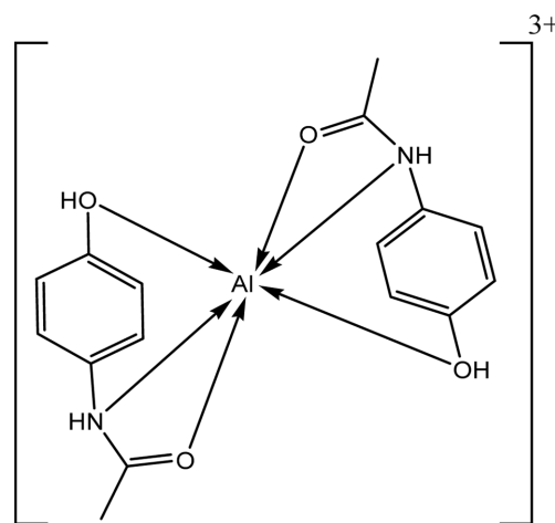
Fig. 21. The structure of Al(III) with PAPA complex.
