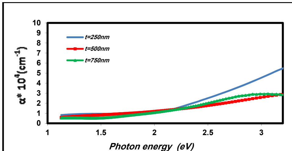
Figure (5) Variation of absorption coefficient with photon energy for AgAlSe 2 thin films at different thicknesses (250, 500, 750) nm.
