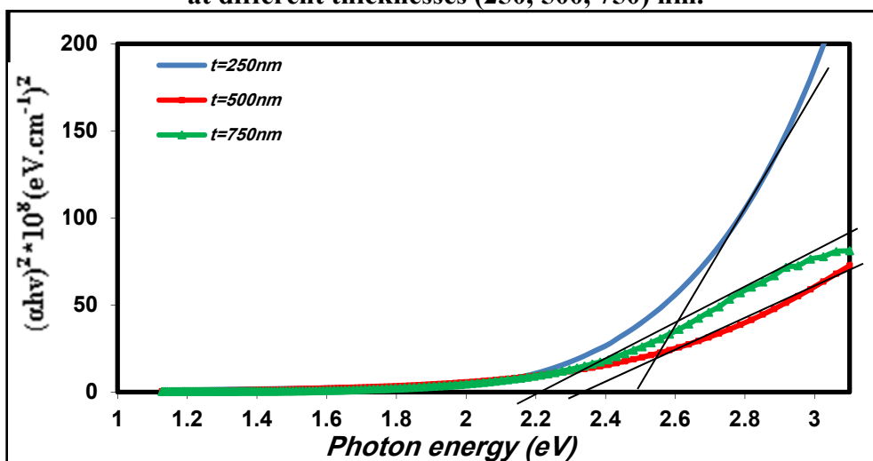
Figure (6) Variation of (\alpha h\nu)^2 with photon energy for AgAlSe 2 thin films at different thicknesses (250, 500, 750) nm.
