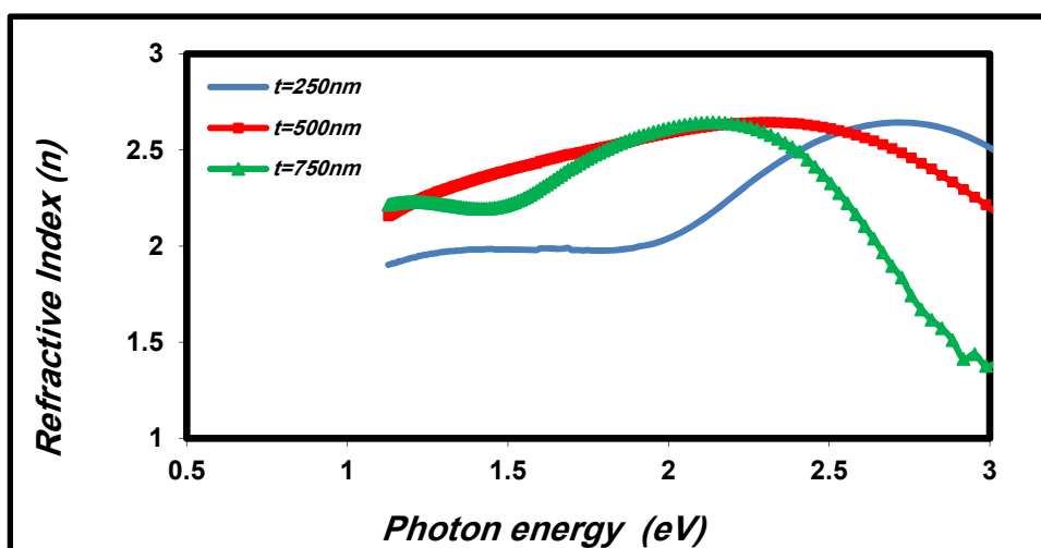
Figure (7) Variation of refractive index with photon energy for AgAlSe 2 thin films at different thicknesses (250, 500, 750) nm.
