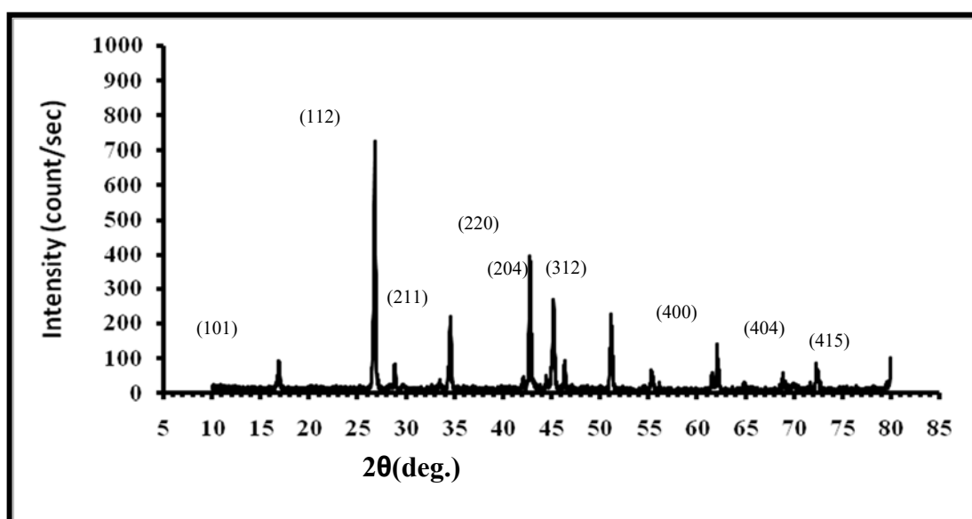
Figure (1) X-ray diffraction pattern of AgAlSe 2 alloy.
