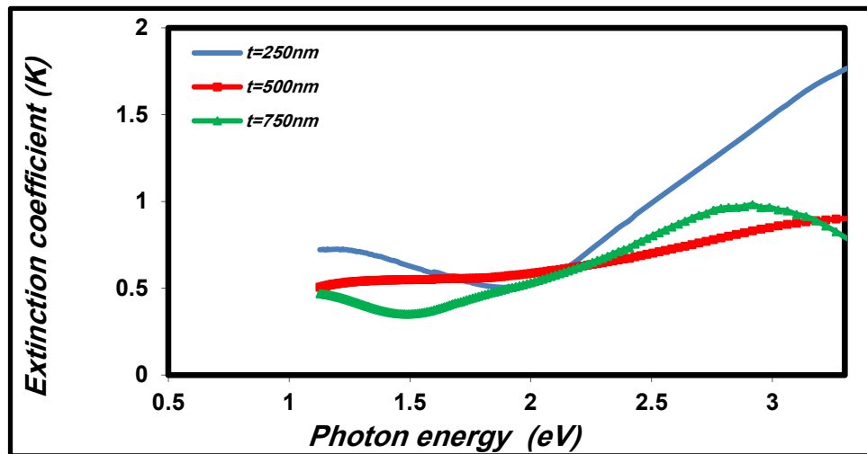
Figure (8) Variation of Extinction coefficient with photon energy for \text{AgAlSe}_2 thin films at different thicknesses (250, 500, 750)nm.
