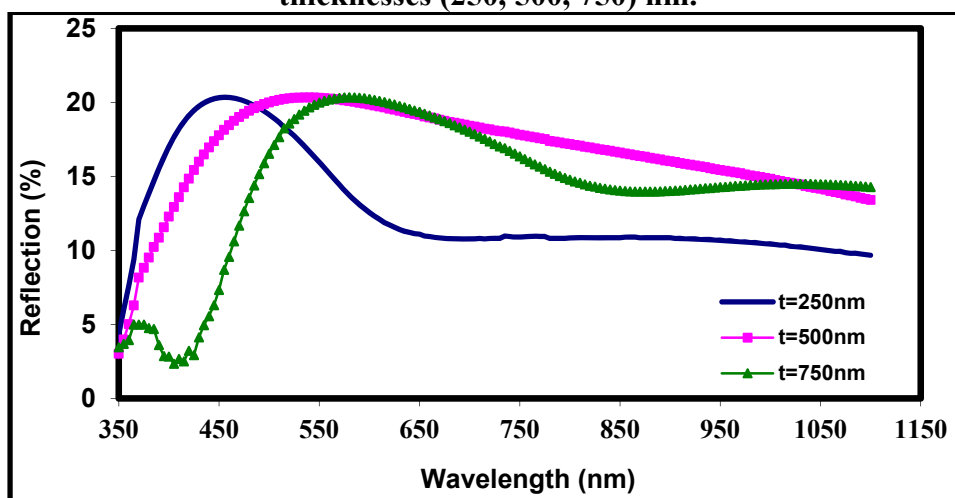
Figure (4) Reflectance spectra for AgAlSe_2 thin films at different thicknesses (250, 500, 750) nm.
