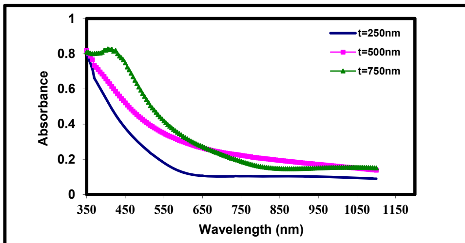
Figure (2) Absorbance spectra for AgAlSe_2 thin films at different thicknesses (250, 500, 750) nm.
