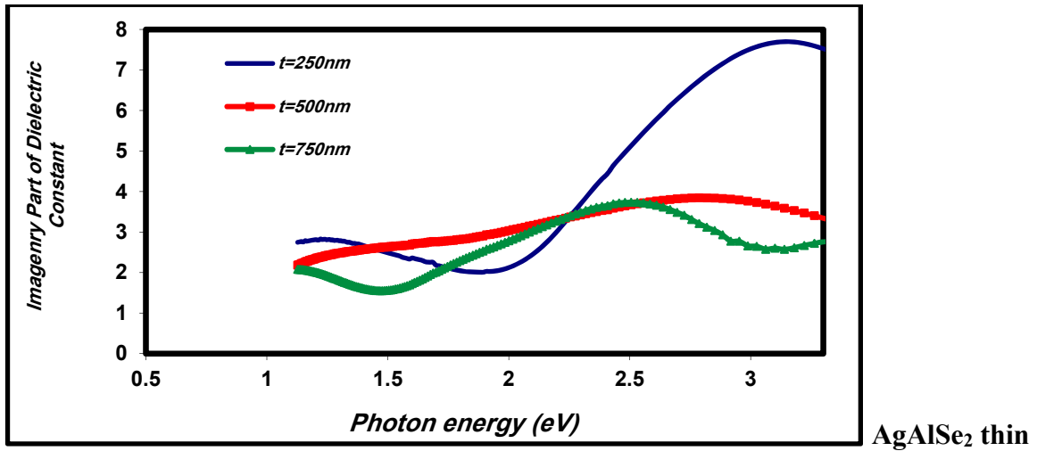
Figure (10) Variation of of imaginary part of dielectric constant with photon energy for films at different thicknesses (250, 500, 750)nm
